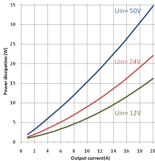
Power dissipation vs output current.
