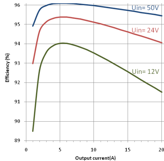
Efficiency vs output current.
